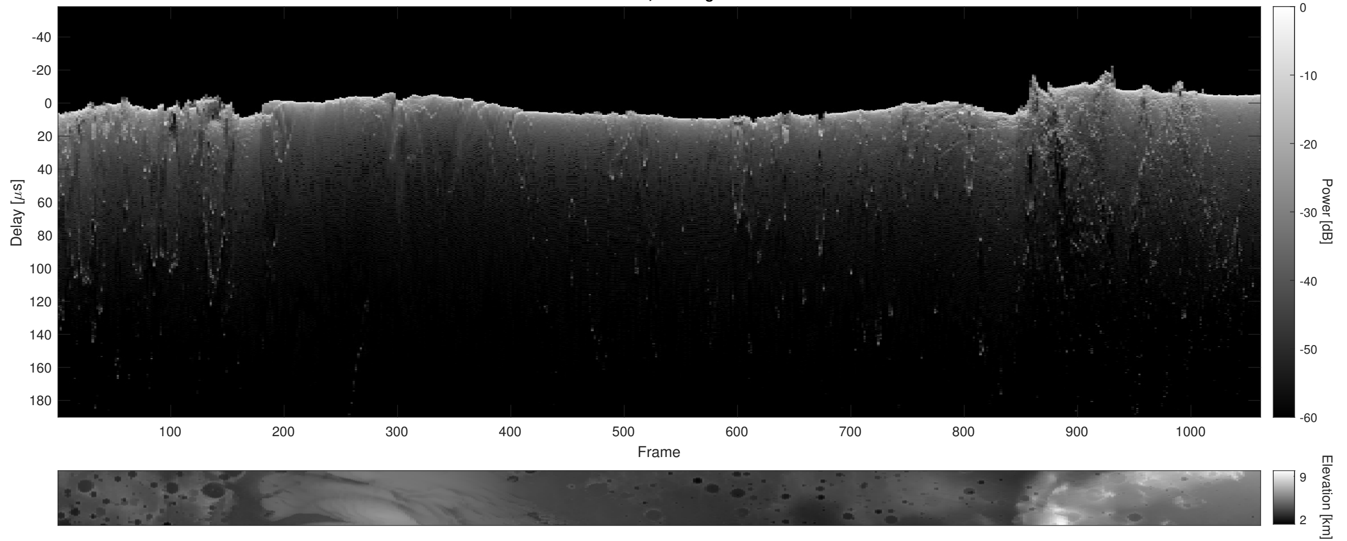
Orbit 2457, Cluttergram
