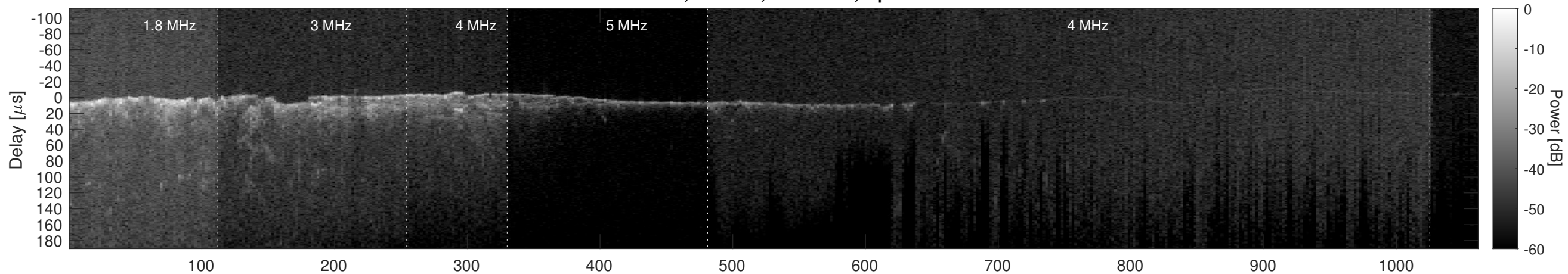
Orbit 2457, Cluttergram
