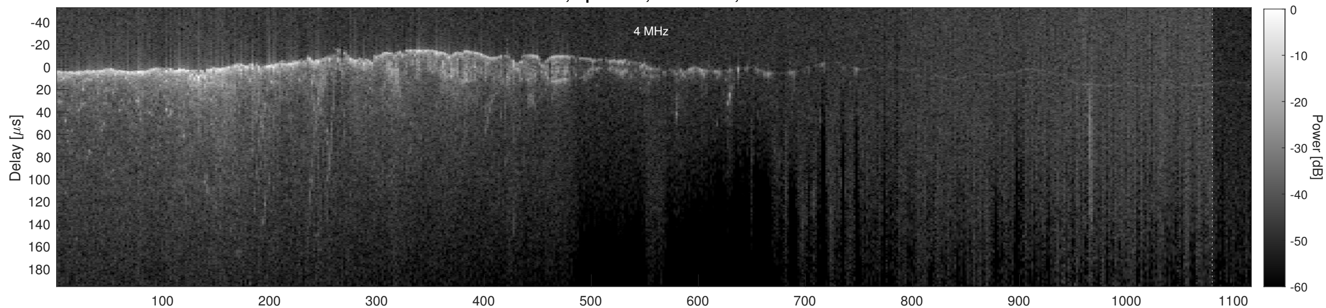
Orbit 2458, Cluttergram
