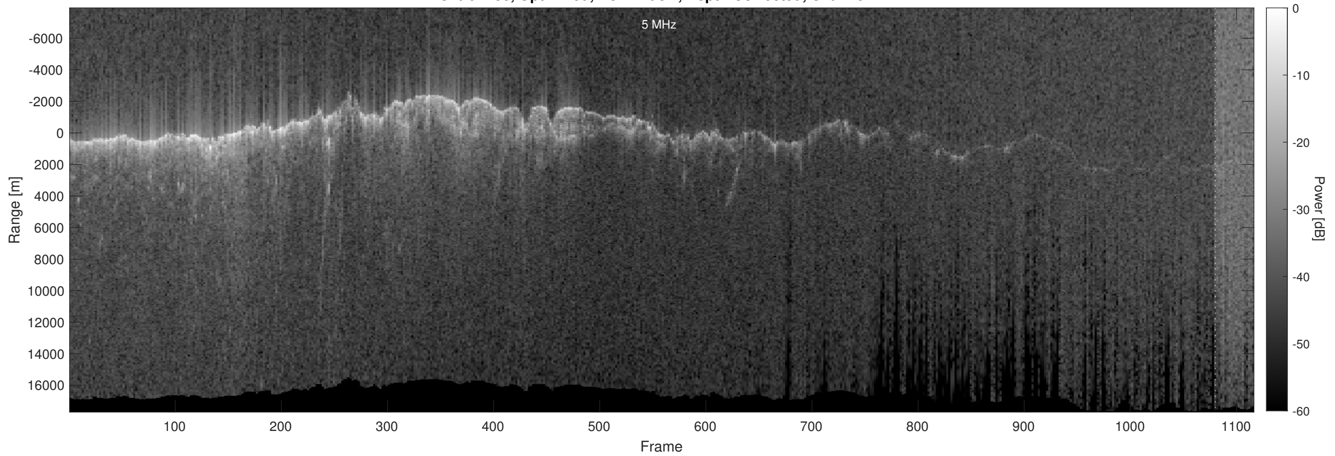
Orbit 2458, Optimized, No Window, Depth-Corrected, Channel 2
