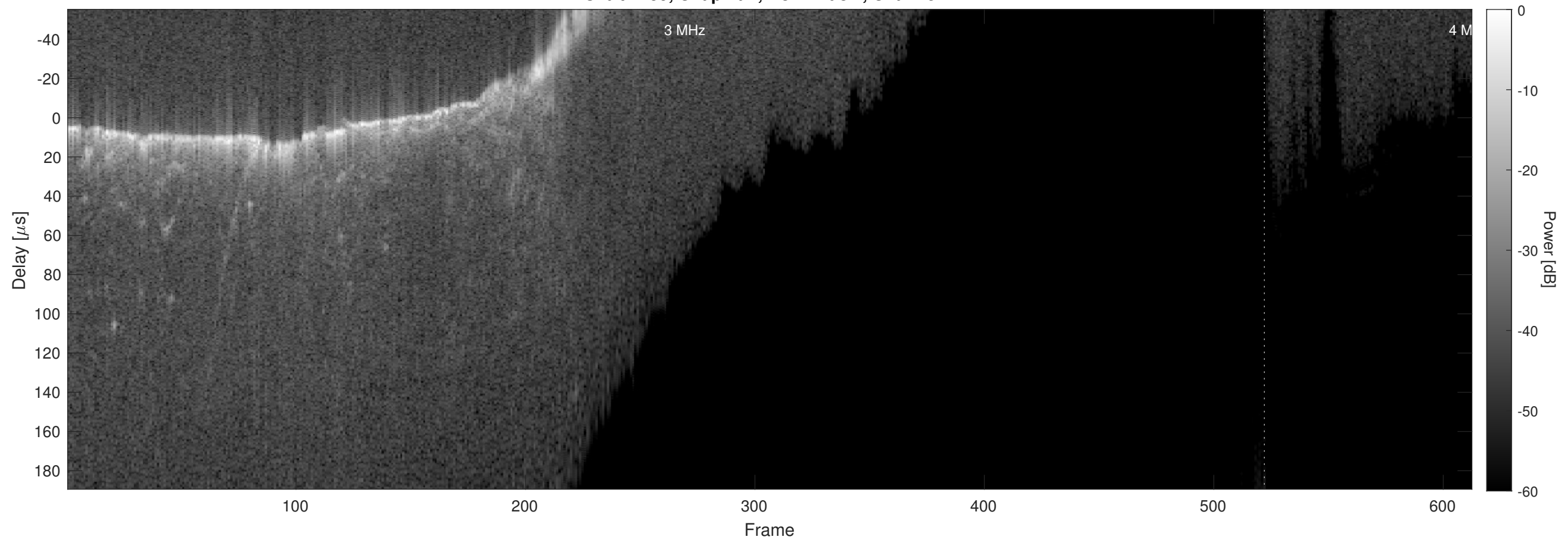
Orbit 2459, Chapman, No Window, Channel 2
