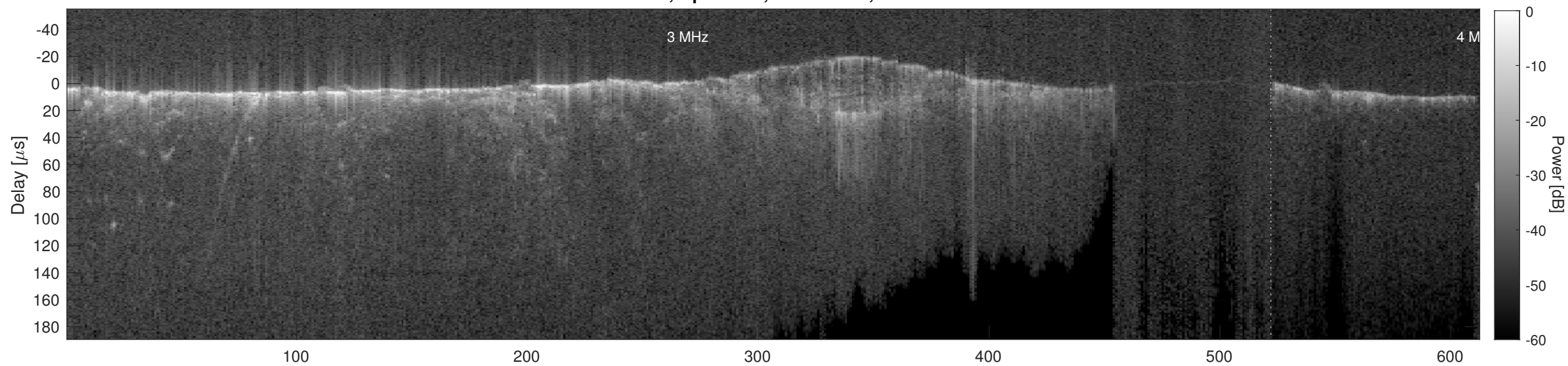
Orbit 2459, Cluttergram
