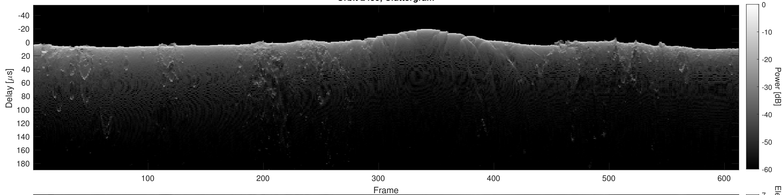
Orbit 2459, Cluttergram
