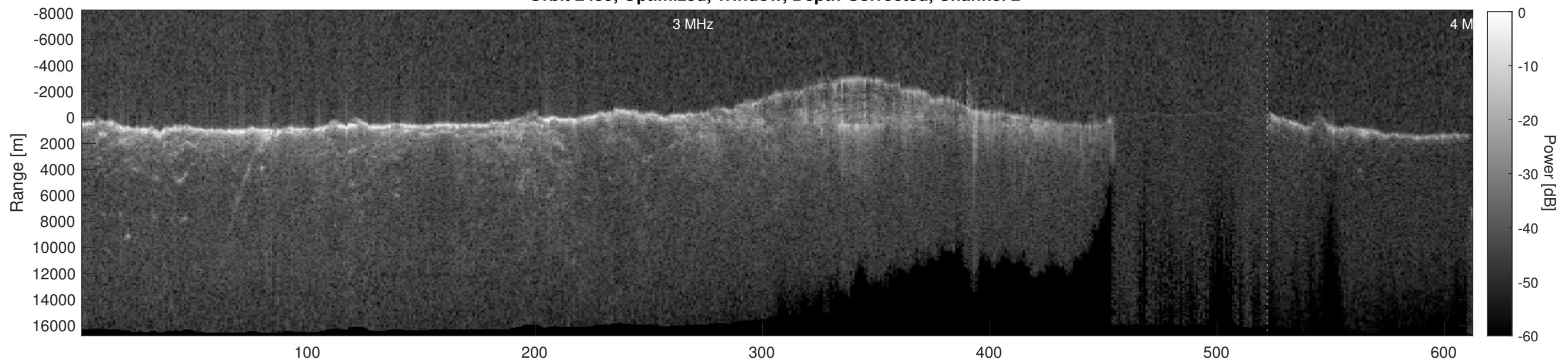
Orbit 2459, Depth-Corrected Cluttergram
