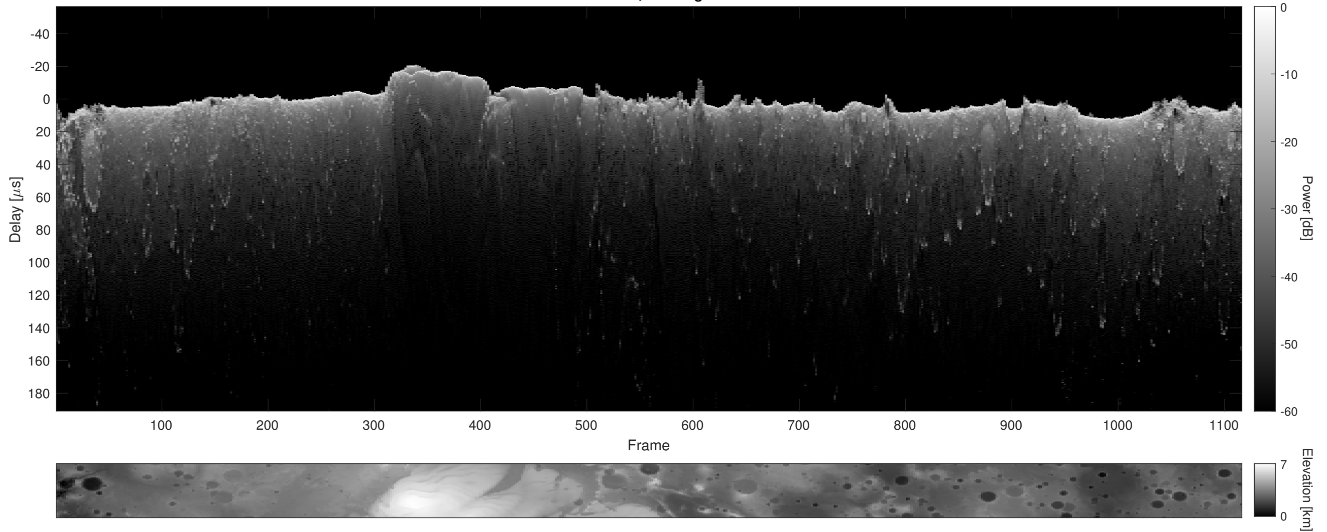
Orbit 2462, Cluttergram
