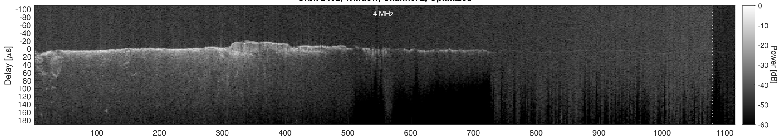
Orbit 2462, Cluttergram
