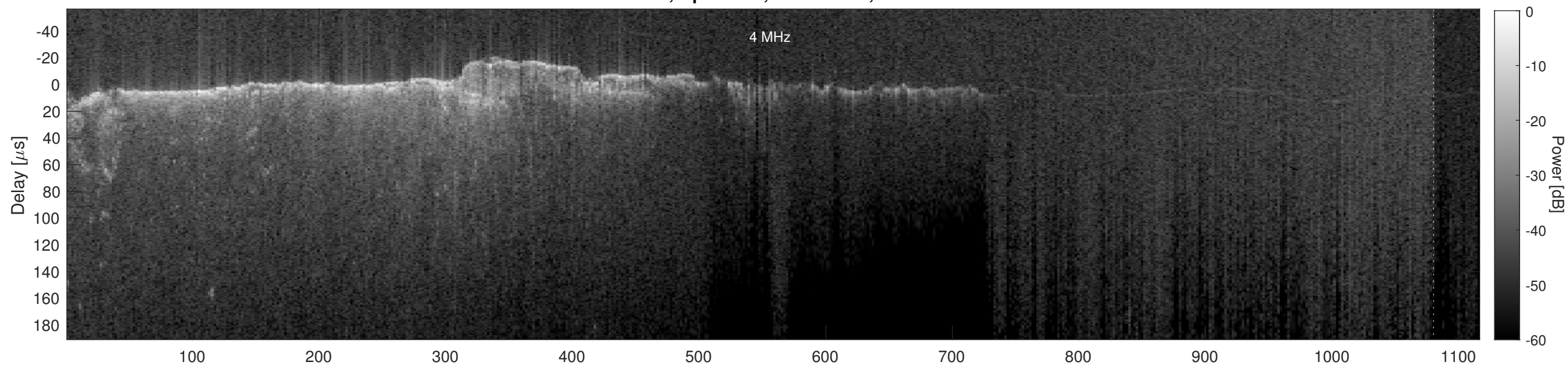
Orbit 2462, Cluttergram
