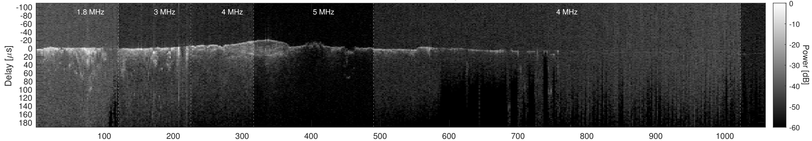
Orbit 2463, Cluttergram
