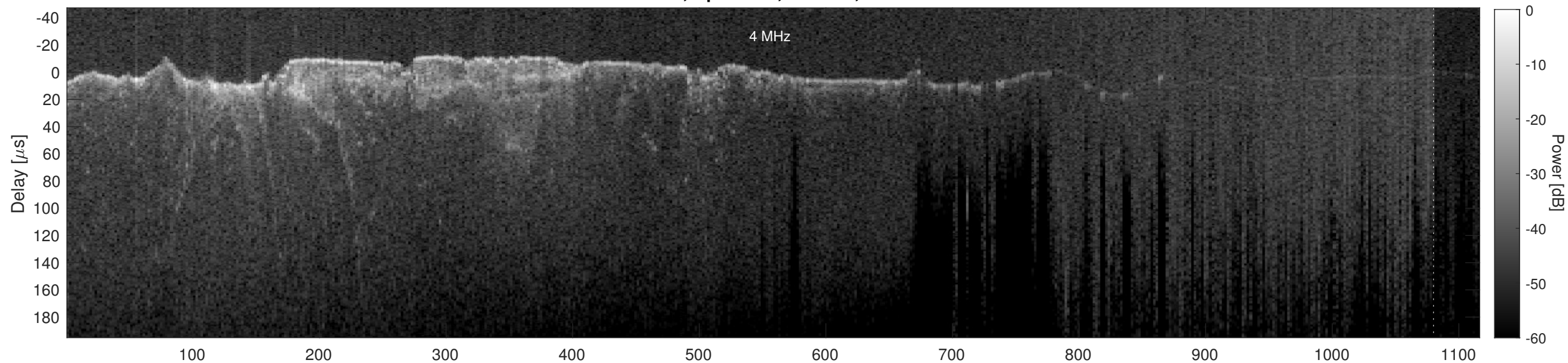
Orbit 2464, Cluttergram
