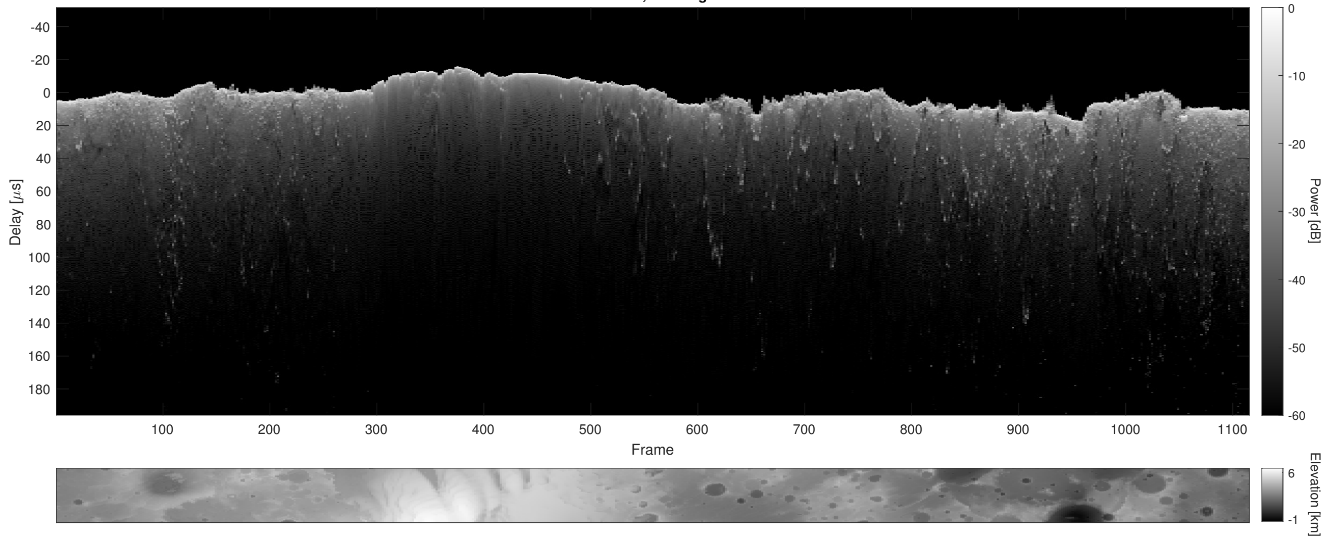
Orbit 2465, Cluttergram
