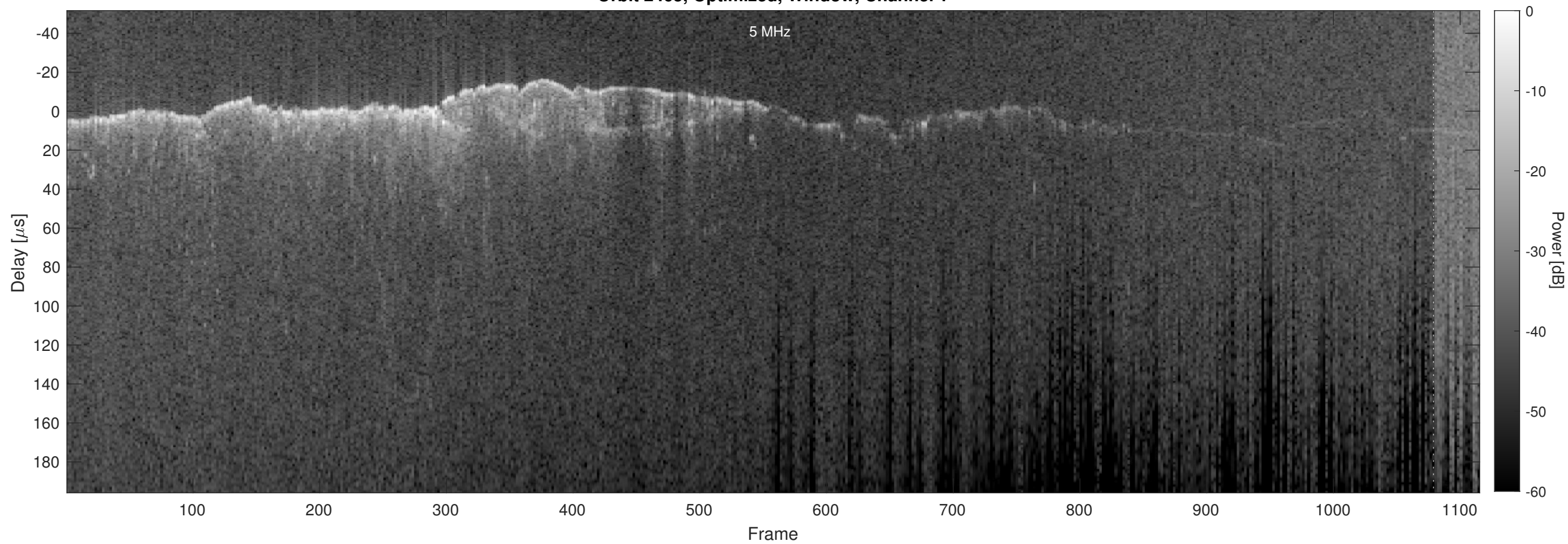
Orbit 2465, Optimized, Window, Channel 2
