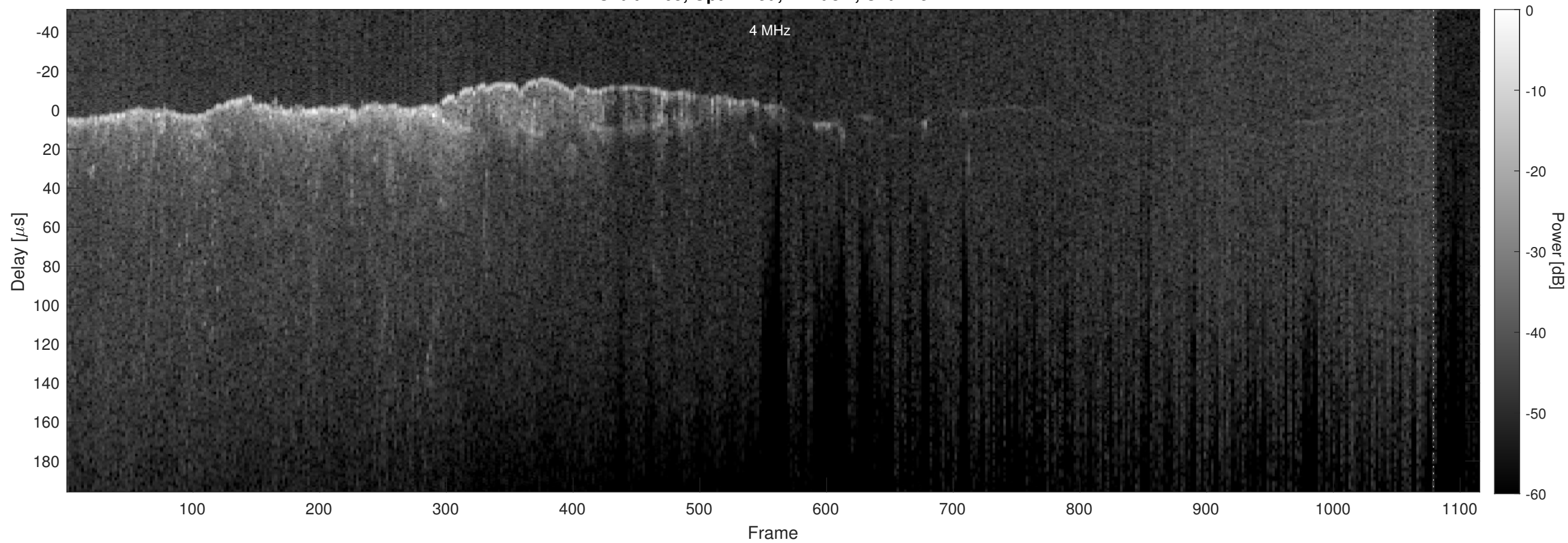
Orbit 2465, Optimized, Window, Channel 2
