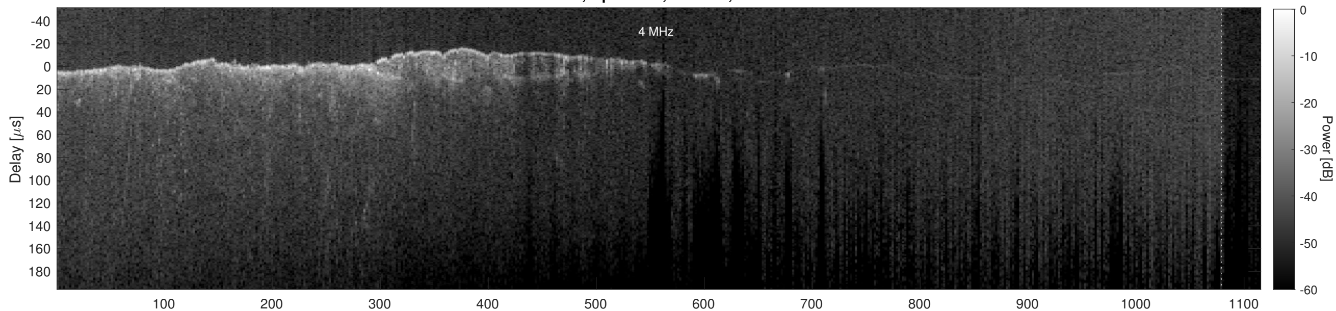
Orbit 2465, Cluttergram
