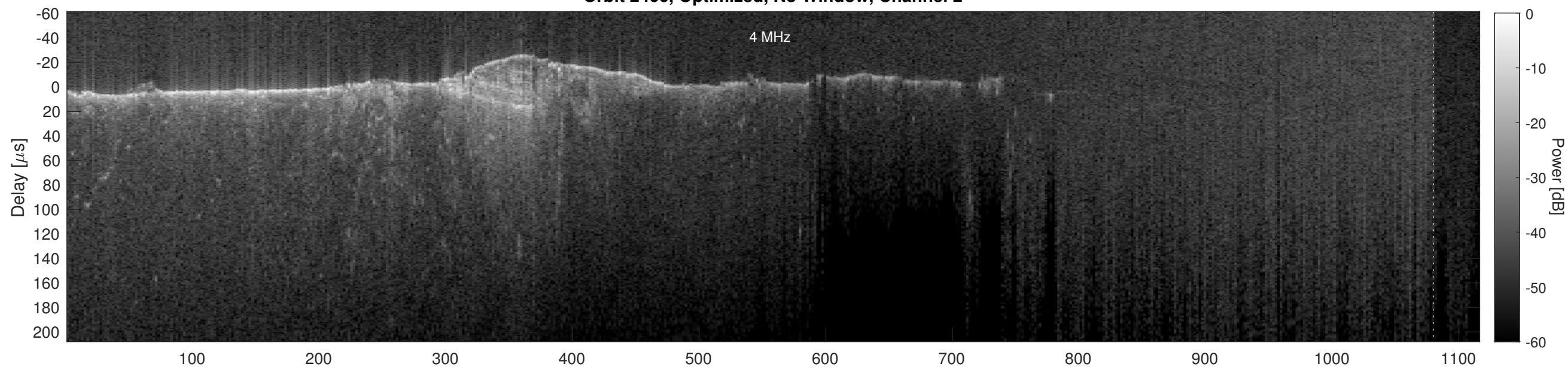
Orbit 2466, Cluttergram
