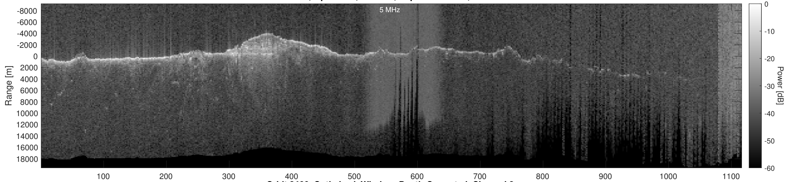
Orbit 2466, Optimized, Window, Depth-Corrected, Channel 2
