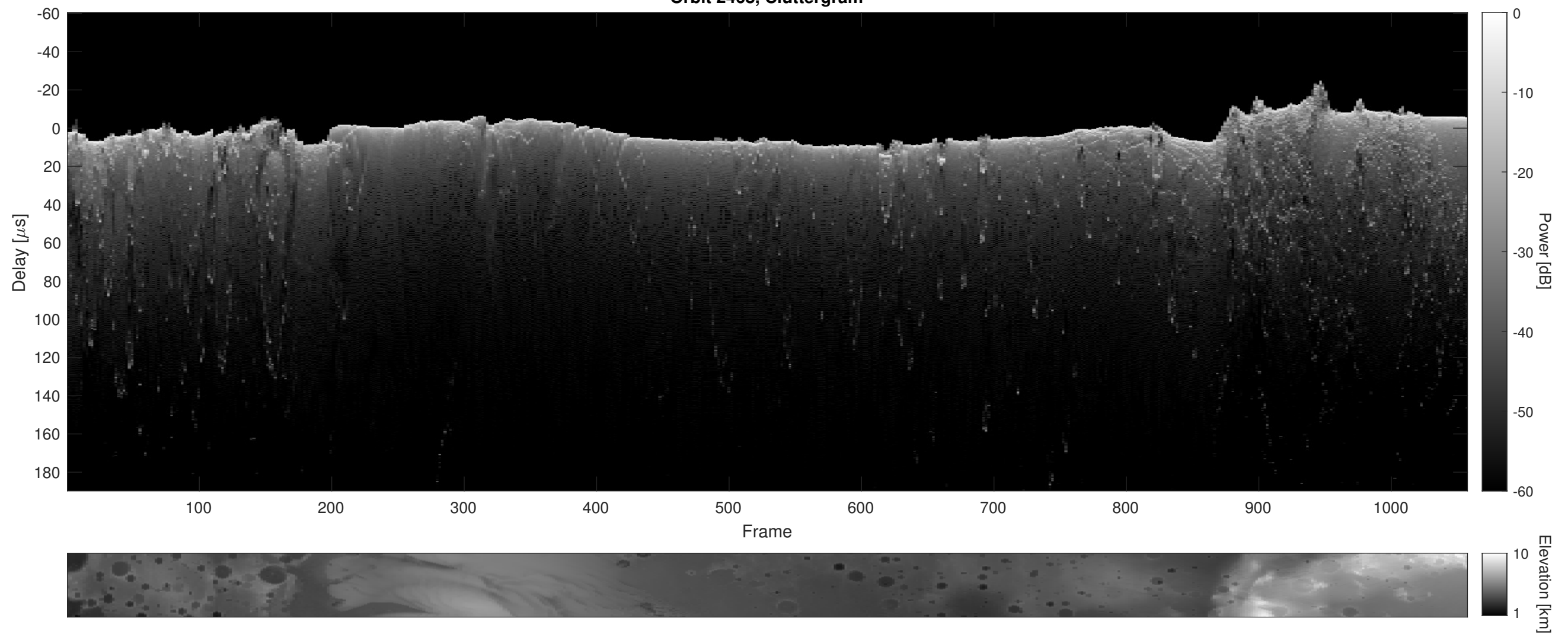
Orbit 2468, Cluttergram
