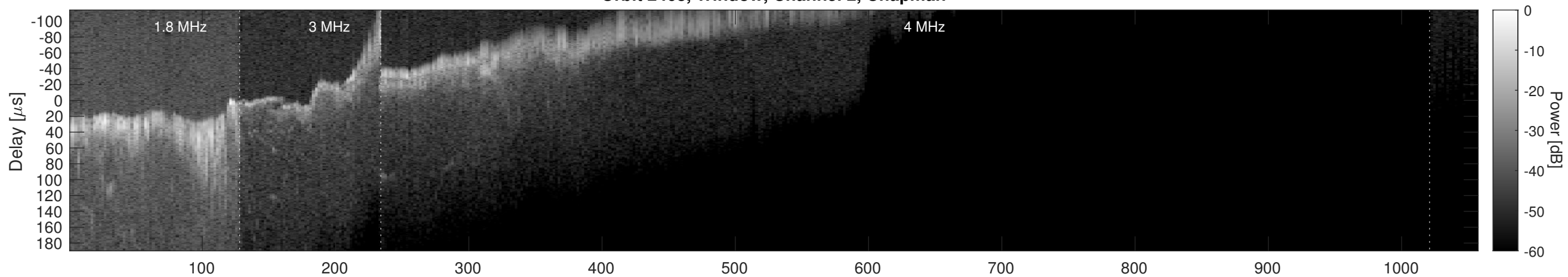
Orbit 2468, Window, Channel 2, Optimized
