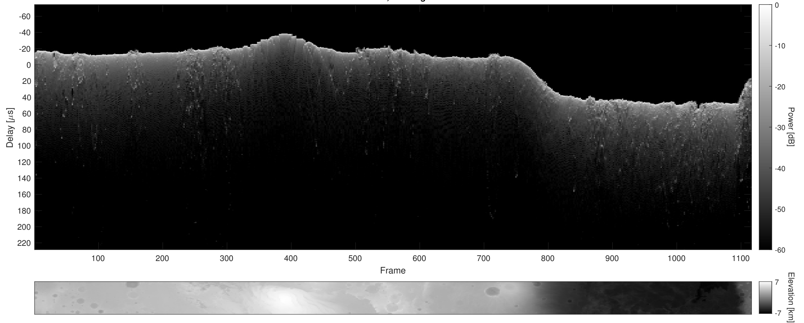
Orbit 2470, Cluttergram
