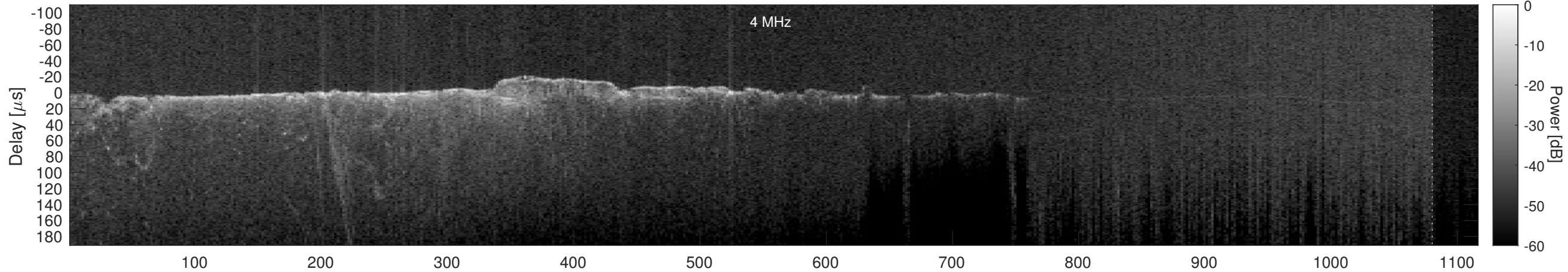
Orbit 2473, Cluttergram
