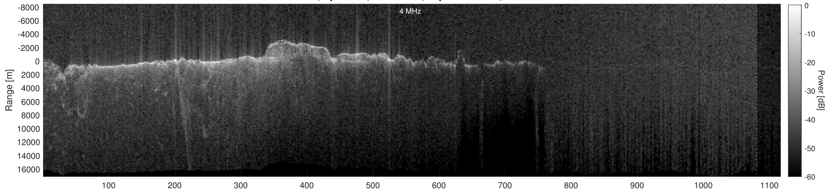
Orbit 2473, Depth-Corrected Cluttergram
