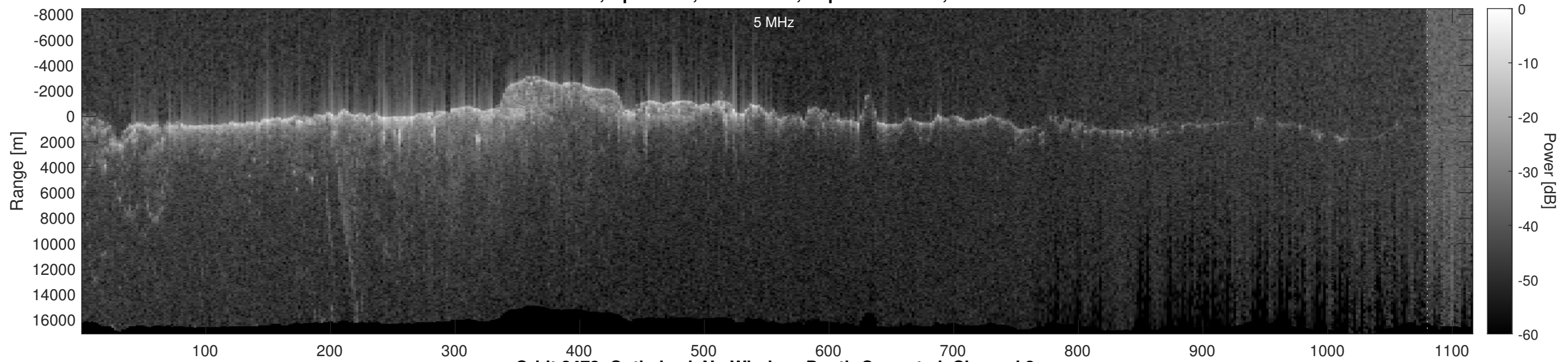
Orbit 2473, Optimized, No Window, Depth-Corrected, Channel 2
