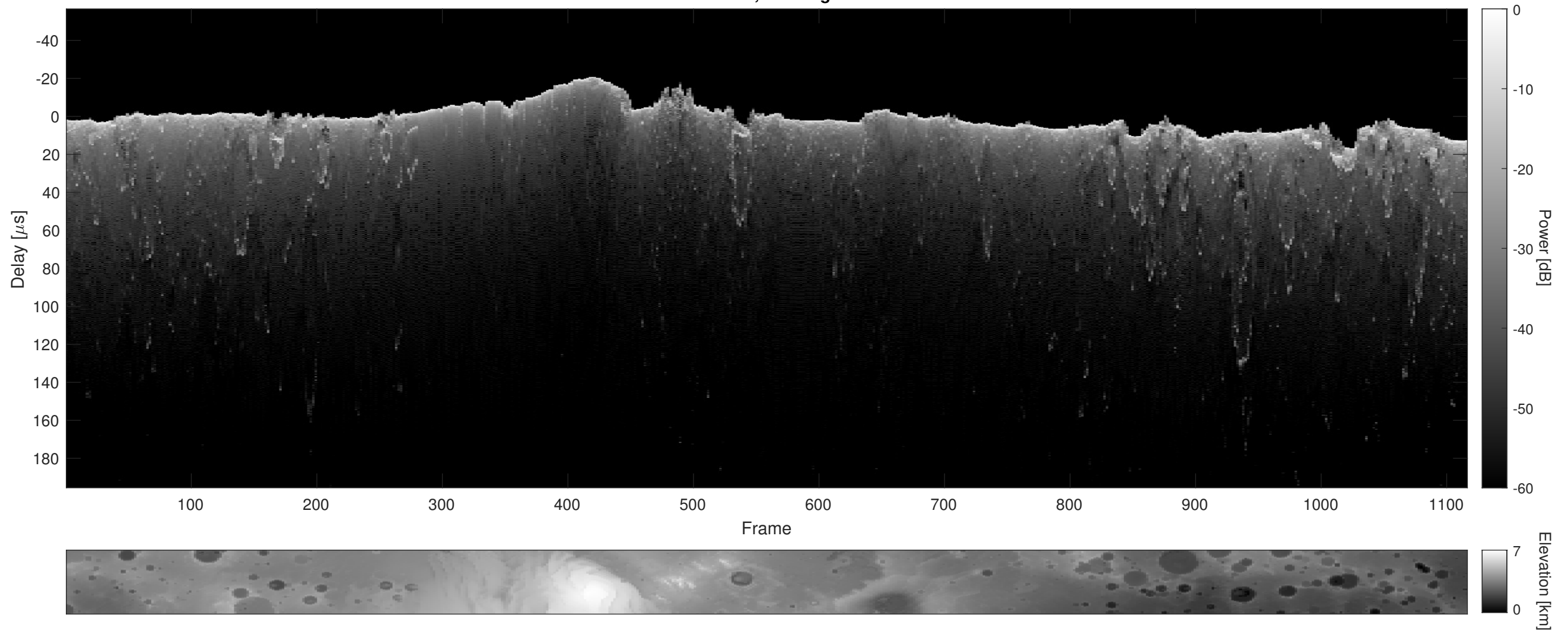
Orbit 2474, Cluttergram
