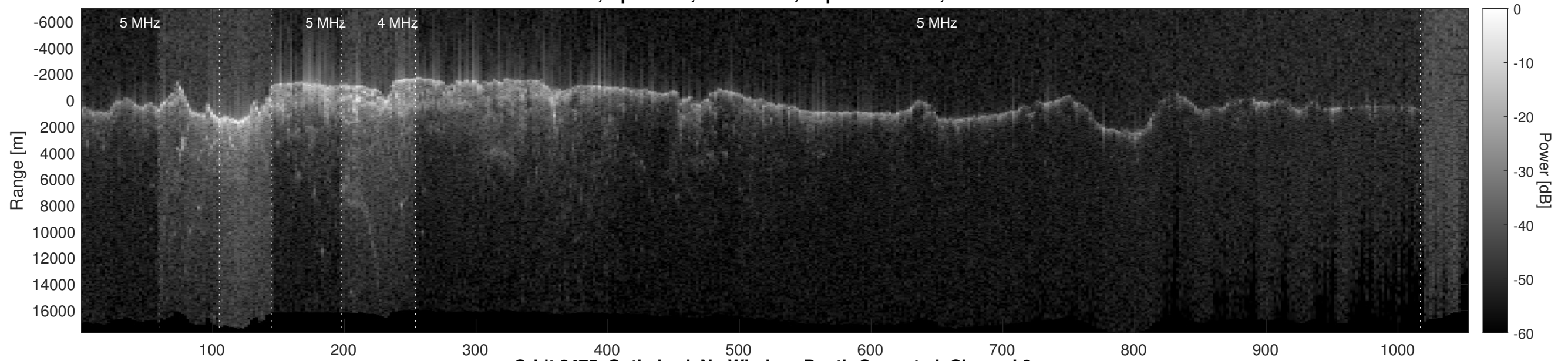
Orbit 2475, Optimized, No Window, Depth-Corrected, Channel 2
