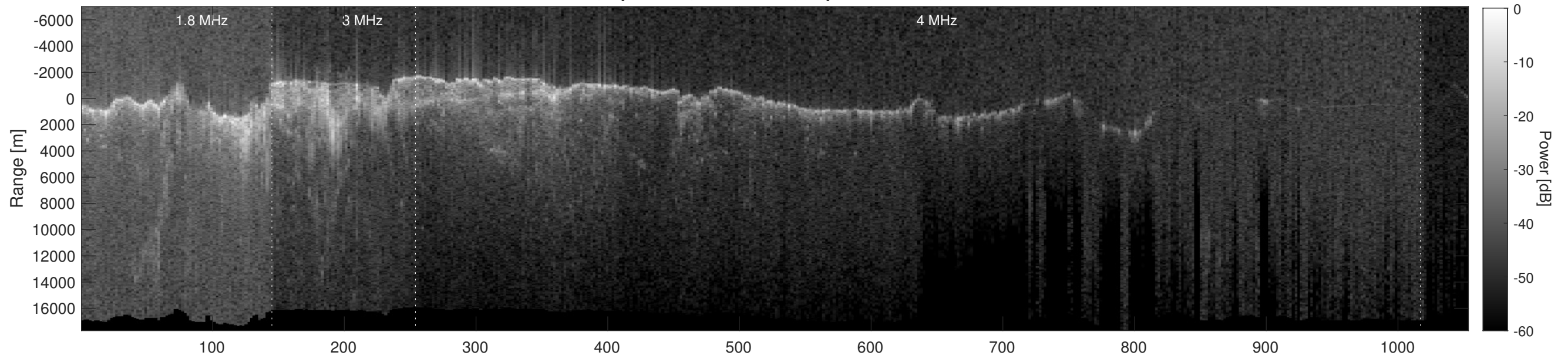
Orbit 2475, Depth-Corrected Cluttergram
