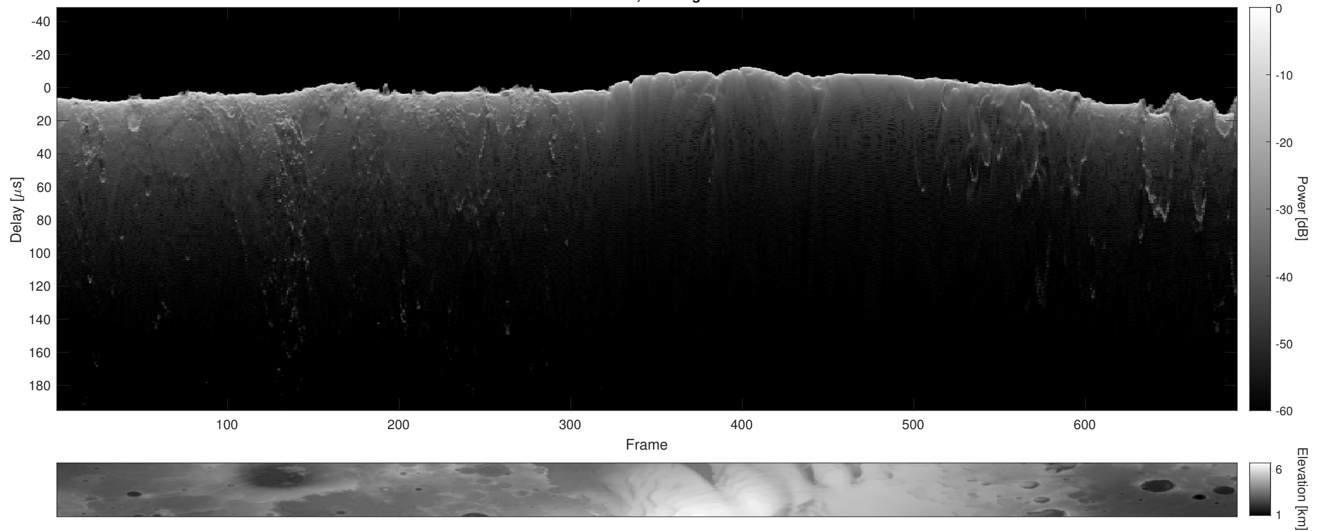
Orbit 2476, Cluttergram
