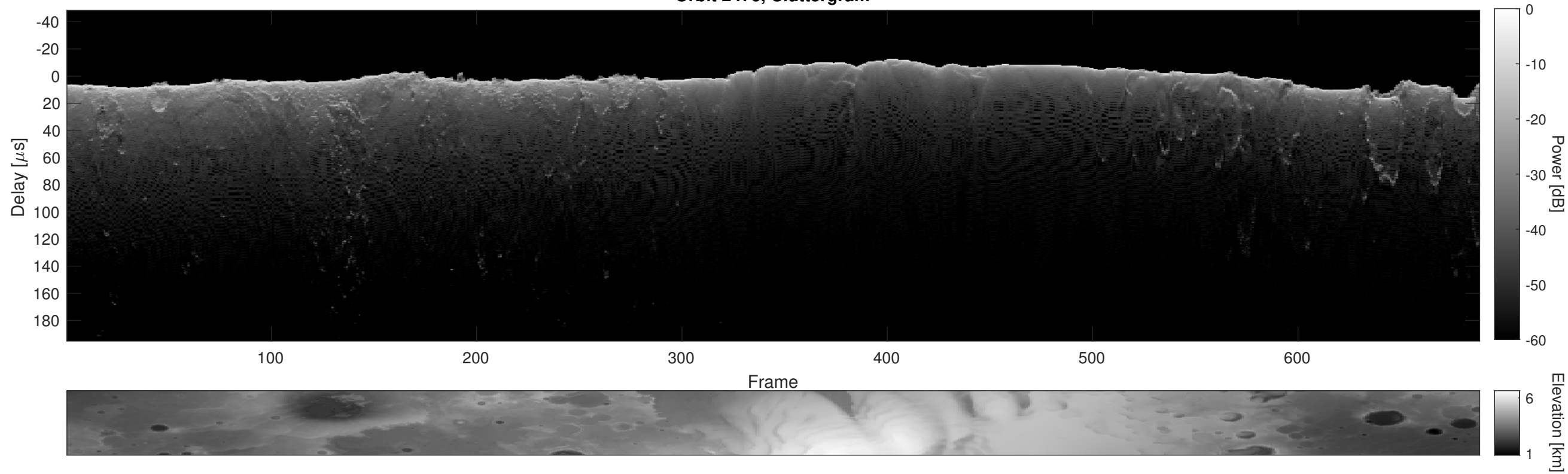
Orbit 2476, Cluttergram
