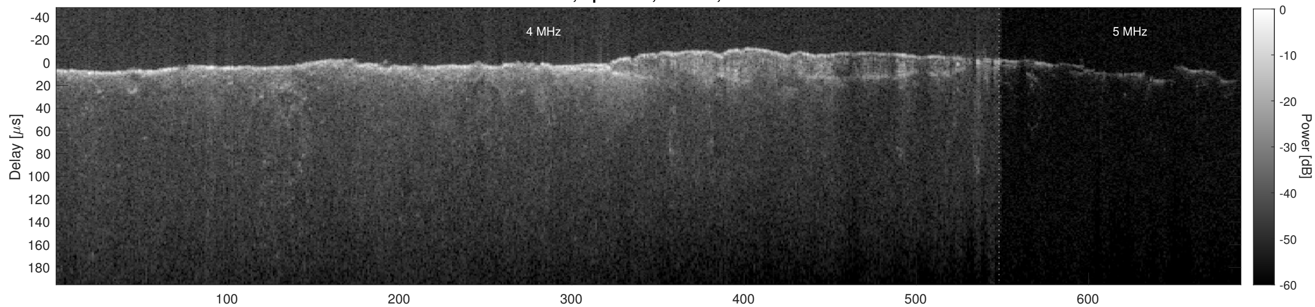
Orbit 2476, Cluttergram
