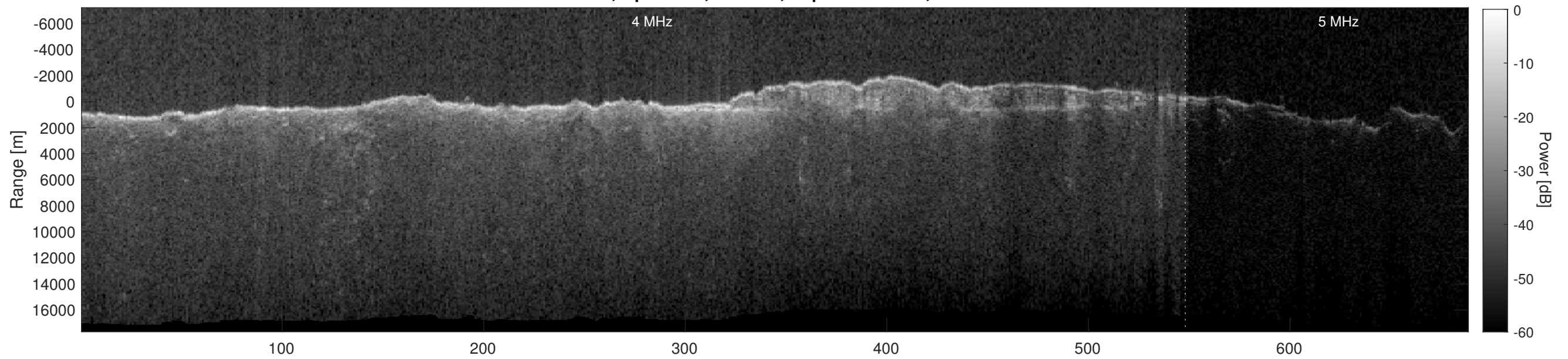
Orbit 2476, Depth-Corrected Cluttergram
