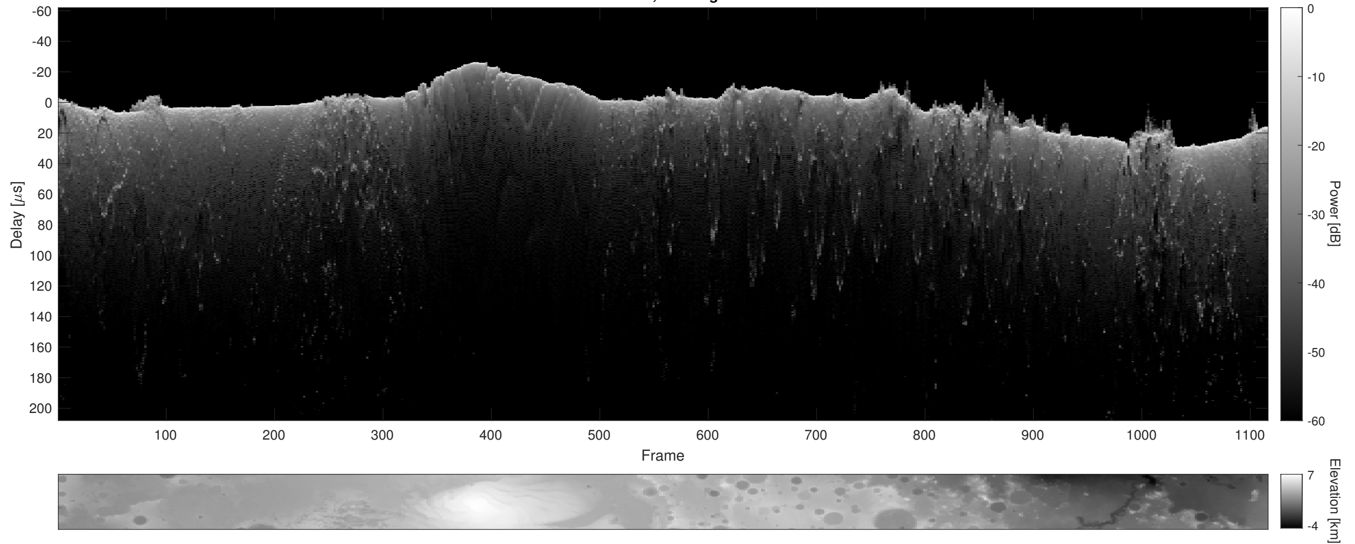
Orbit 2477, Cluttergram
