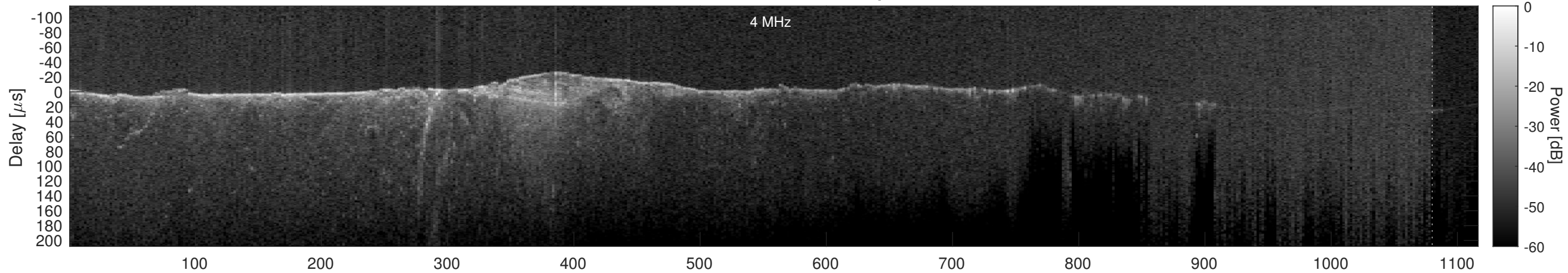
Orbit 2477, Cluttergram
