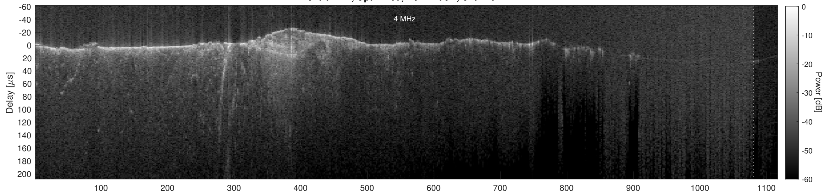
Orbit 2477, Cluttergram
