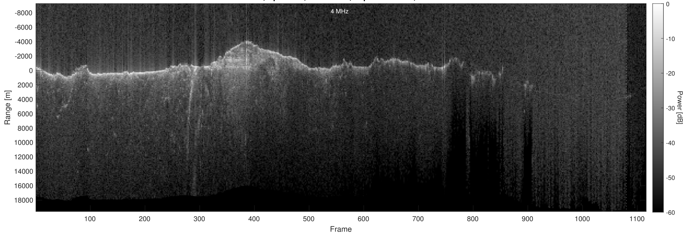
Orbit 2477, Optimized, No Window, Depth-Corrected, Channel 2
