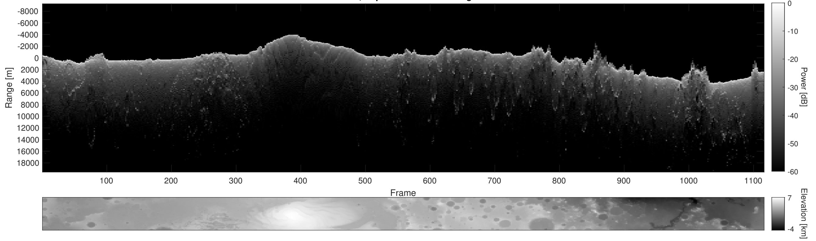
Orbit 2477, Depth-Corrected Cluttergram
