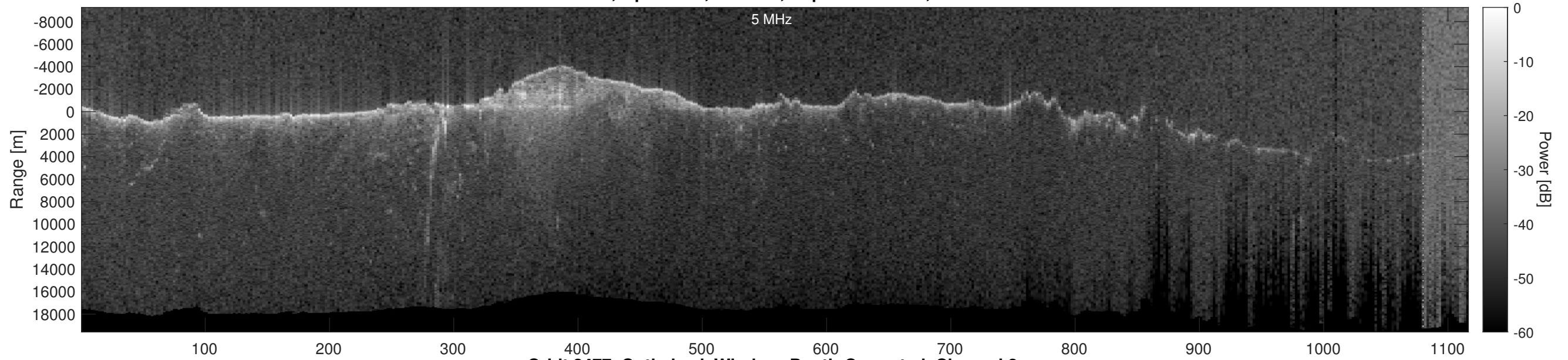
Orbit 2477, Optimized, Window, Depth-Corrected, Channel 2
