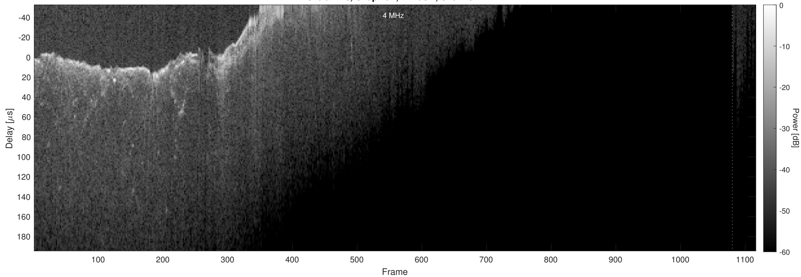
Orbit 2478, Chapman, Window, Channel 2
