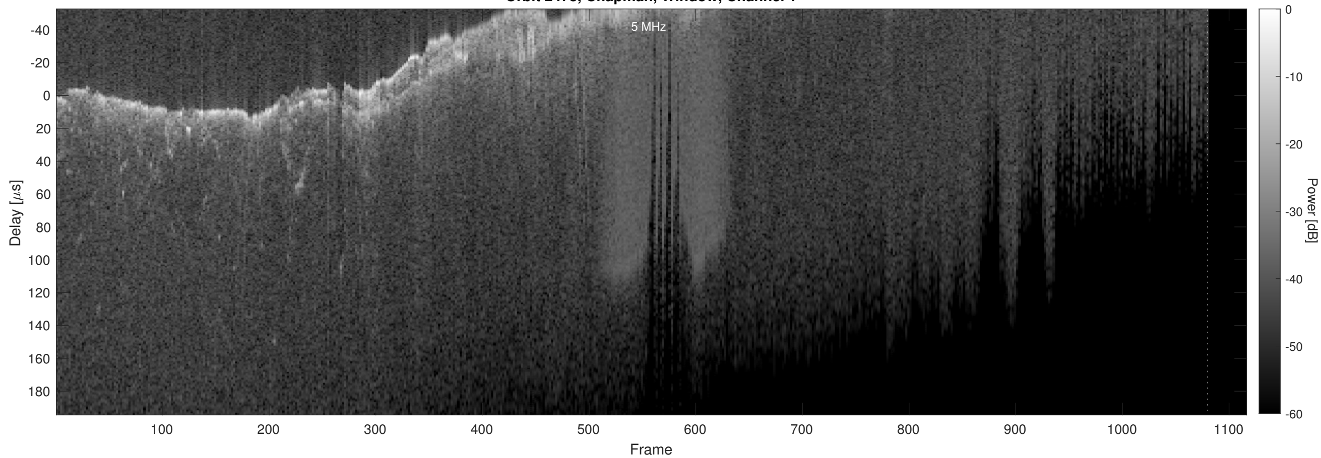
Orbit 2478, Chapman, Window, Channel 2
