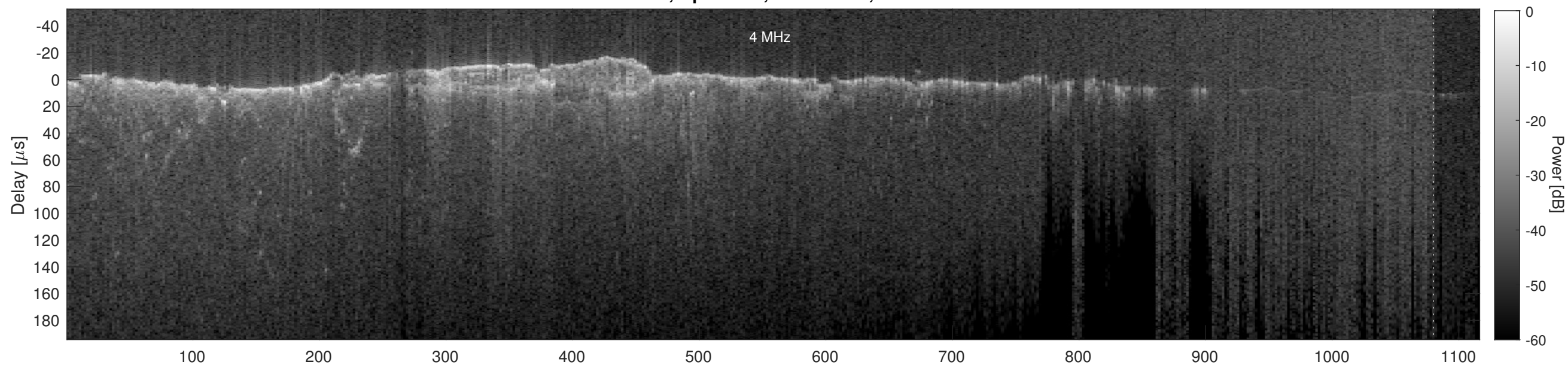
Orbit 2478, Cluttergram
