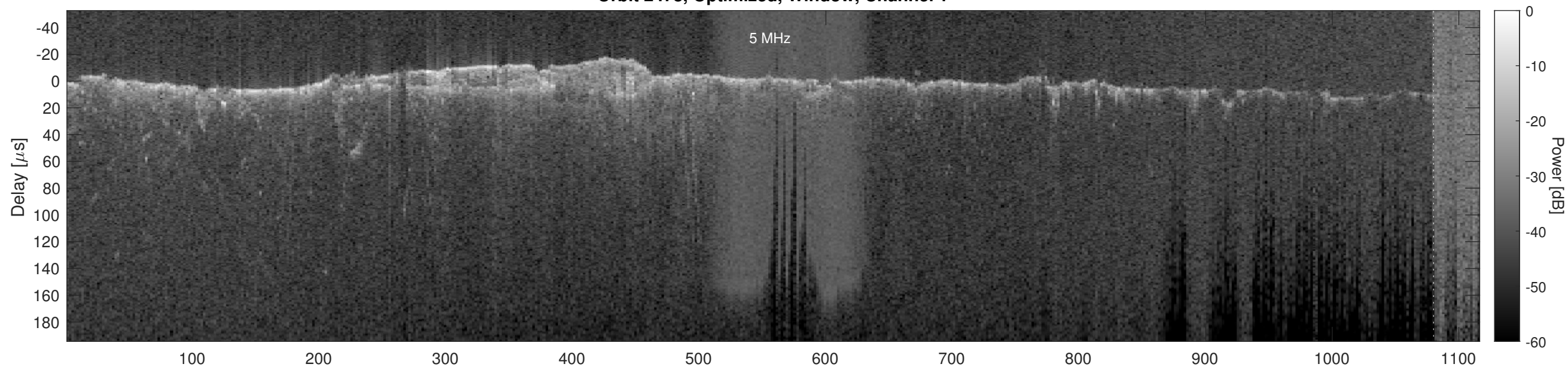
Orbit 2478, Optimized, Window, Channel 2
