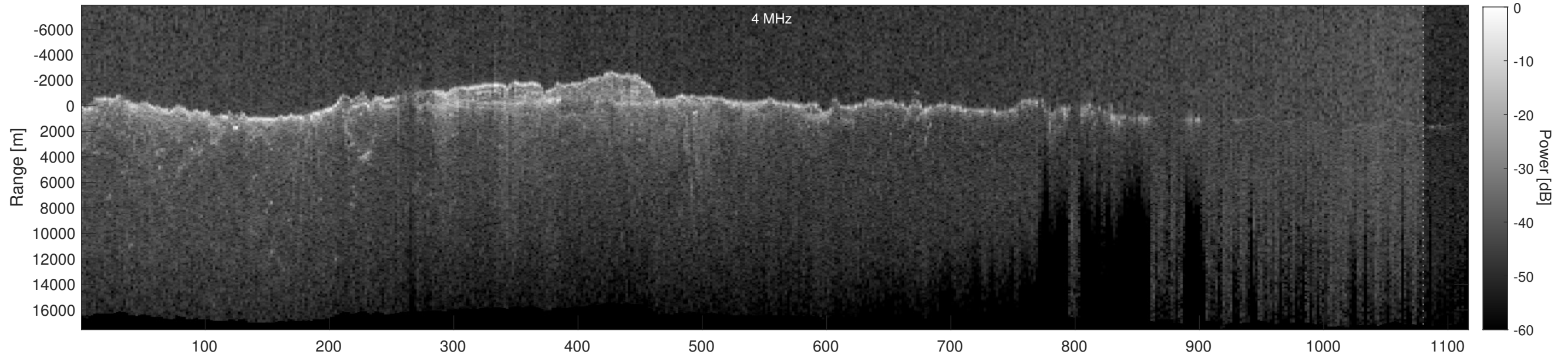
Orbit 2478, Depth-Corrected Cluttergram
