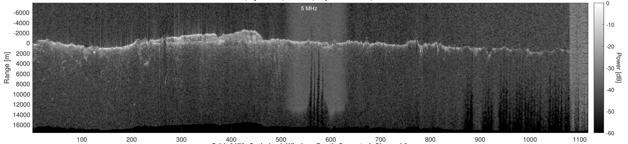
Orbit 2478, Optimized, Window, Depth-Corrected, Channel 2
