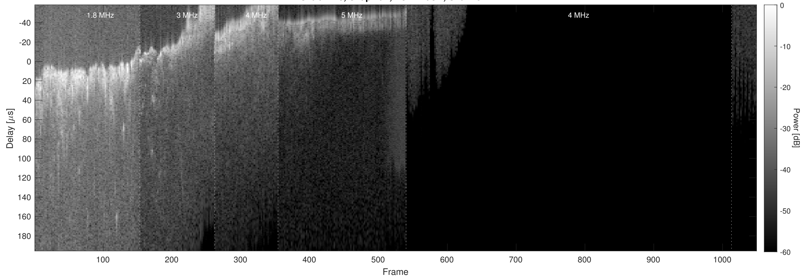
Orbit 2479, Chapman, No Window, Channel 2
