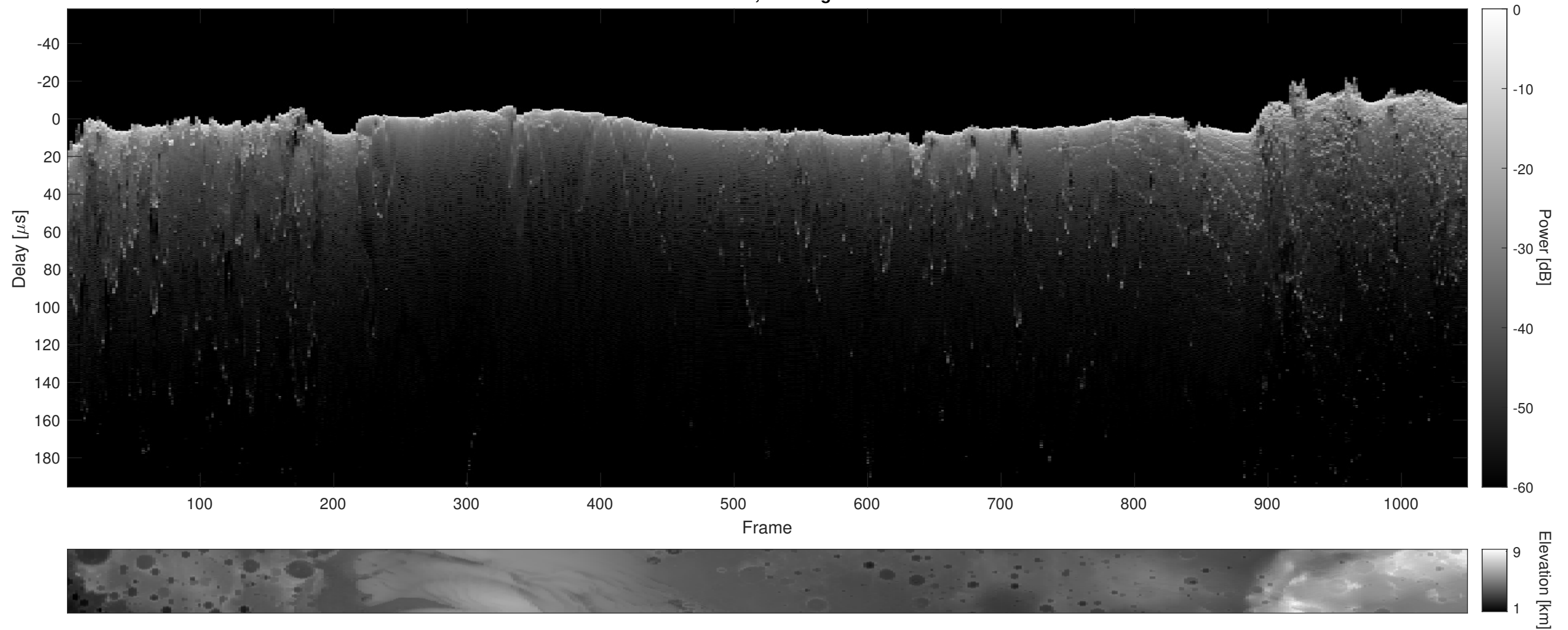
Orbit 2479, Cluttergram
