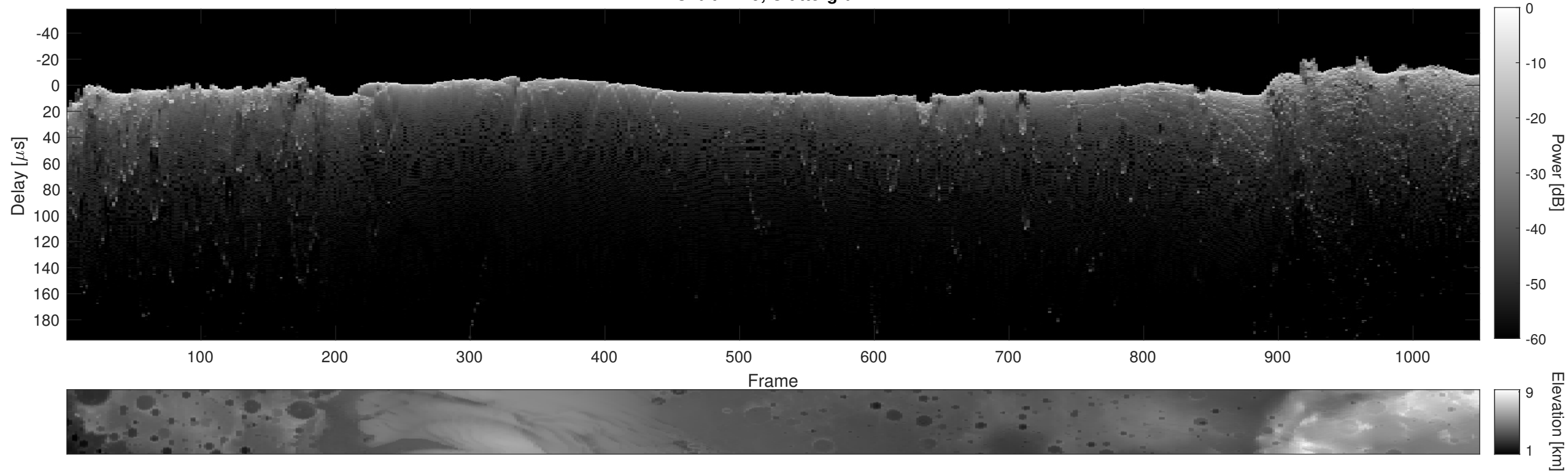
Orbit 2479, Cluttergram
