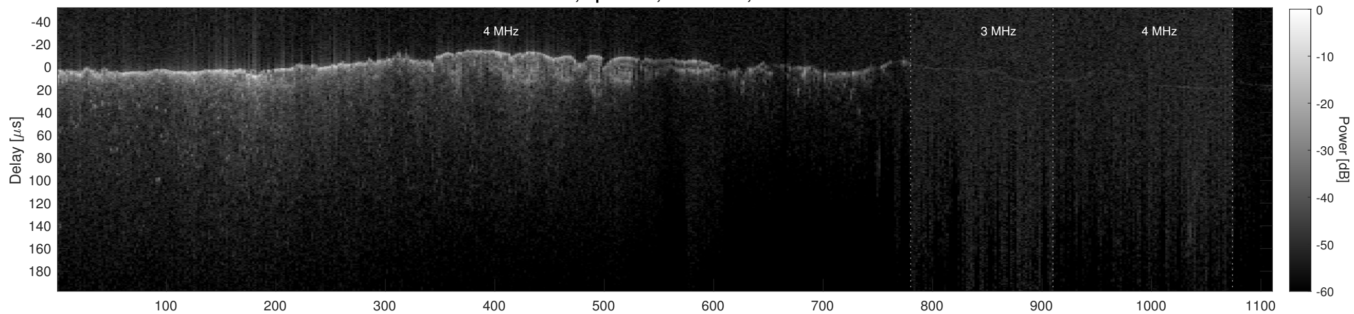
Orbit 2480, Cluttergram
