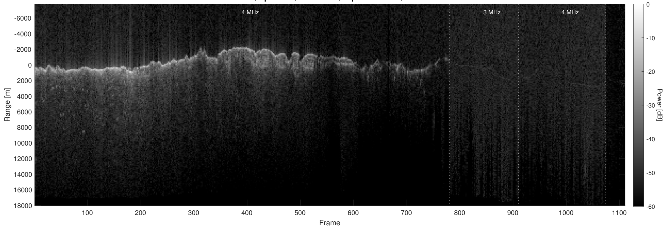
Orbit 2480, Optimized, No Window, Depth-Corrected, Channel 2
