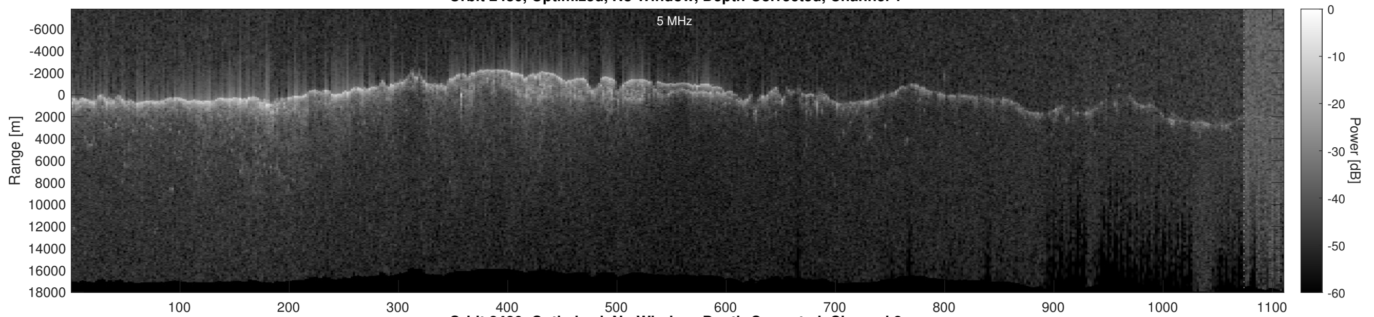
Orbit 2480, Optimized, No Window, Depth-Corrected, Channel 2
