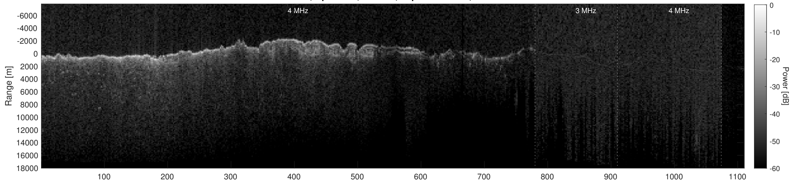
Orbit 2480, Depth-Corrected Cluttergram
