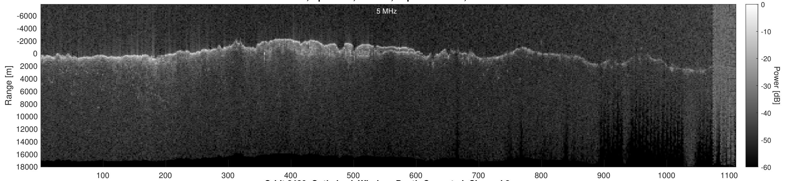
Orbit 2480, Optimized, Window, Depth-Corrected, Channel 2
