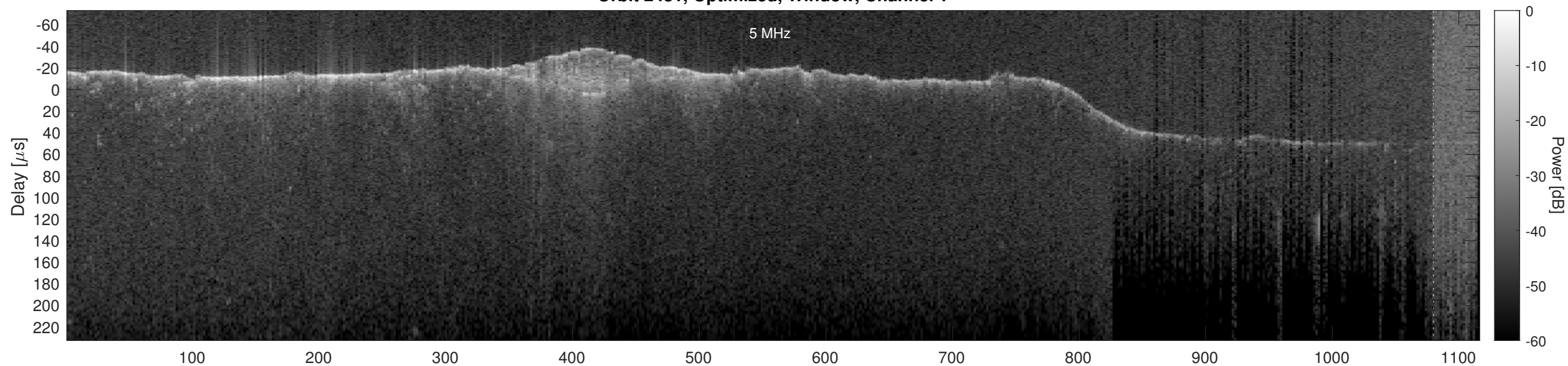
Orbit 2481, Optimized, Window, Channel 2
