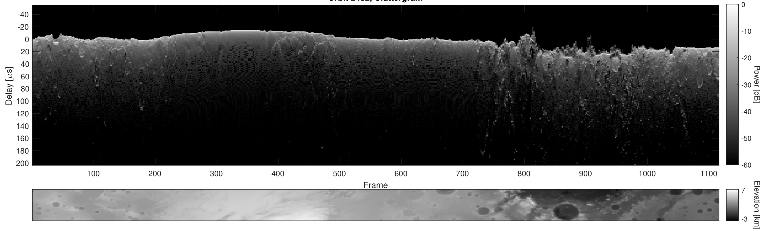
Orbit 2482, Cluttergram
