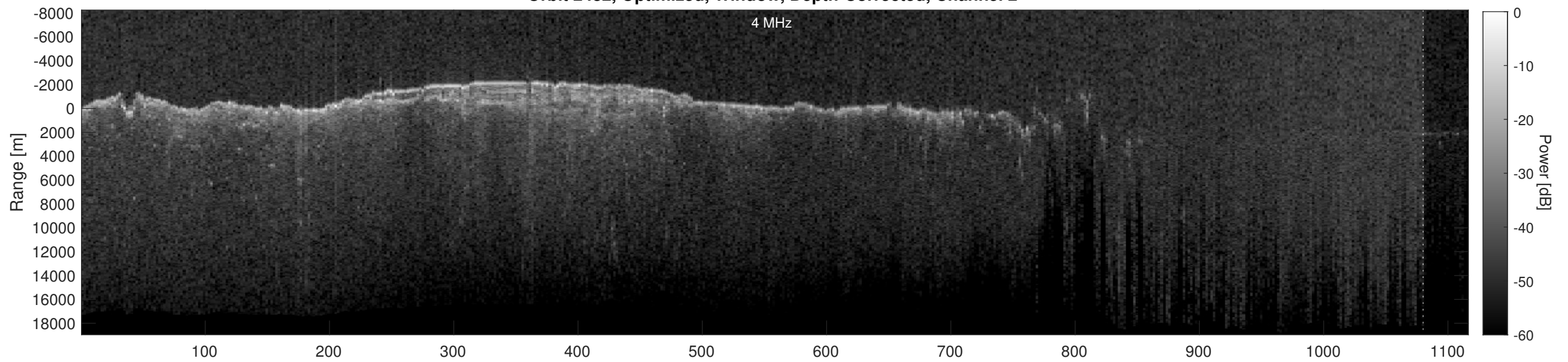
Orbit 2482, Depth-Corrected Cluttergram
