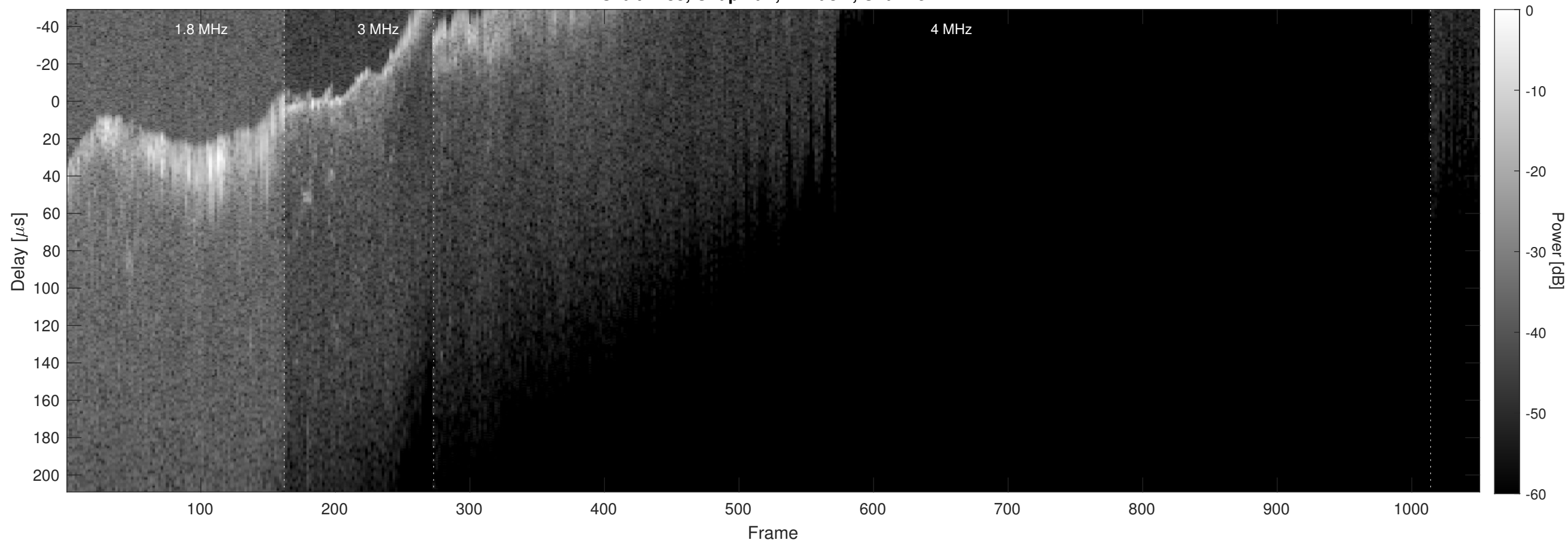
Orbit 2483, Chapman, Window, Channel 2
