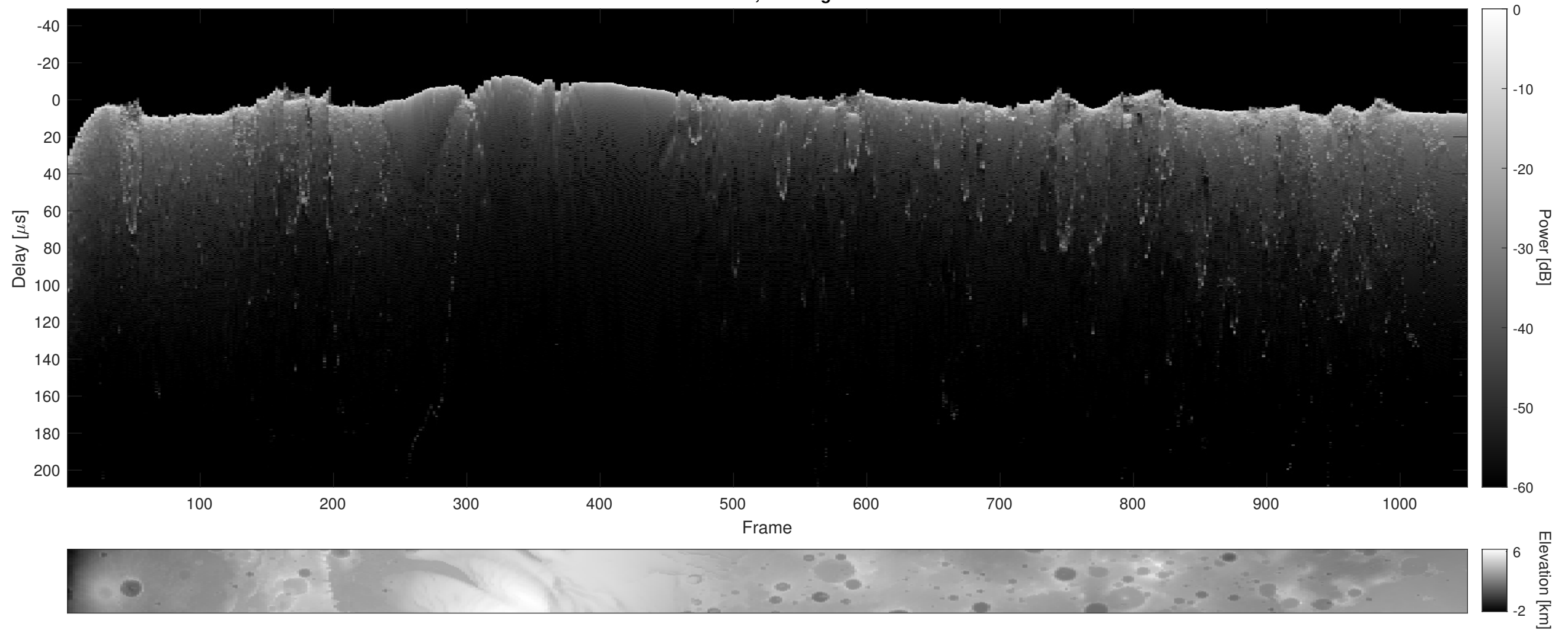
Orbit 2483, Cluttergram
